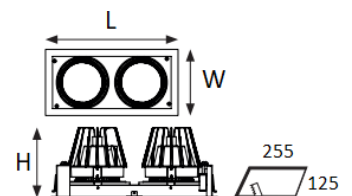
EDL2X10W
