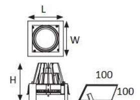
EDL2X10W
